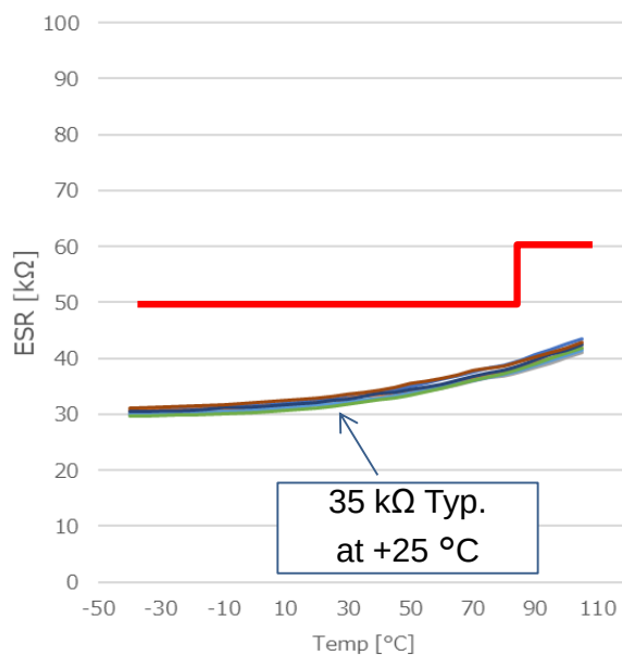
FC2012AN Temp. Characteristics (ESR)
