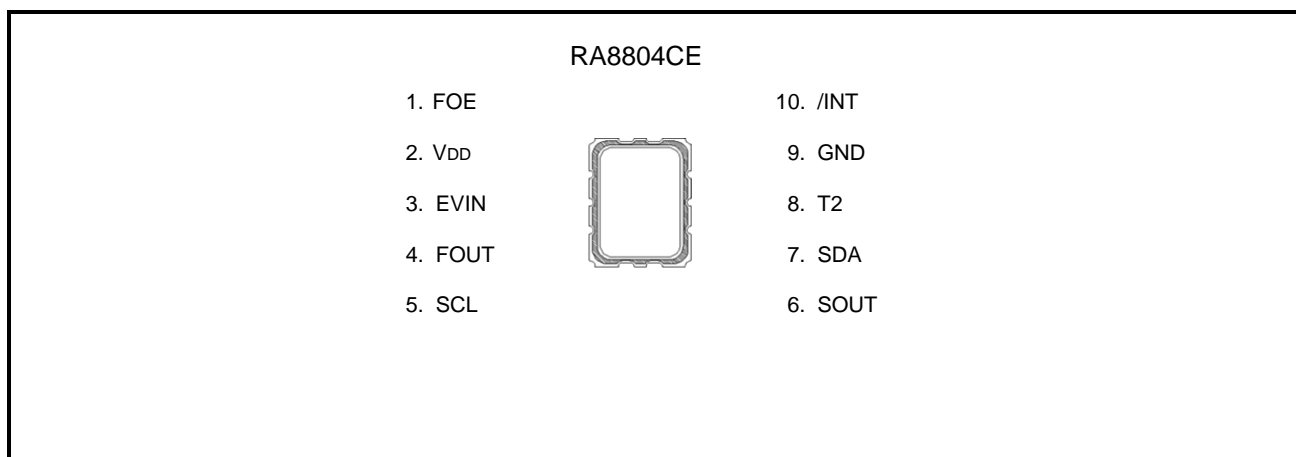
Figure 3 Pin Layout
