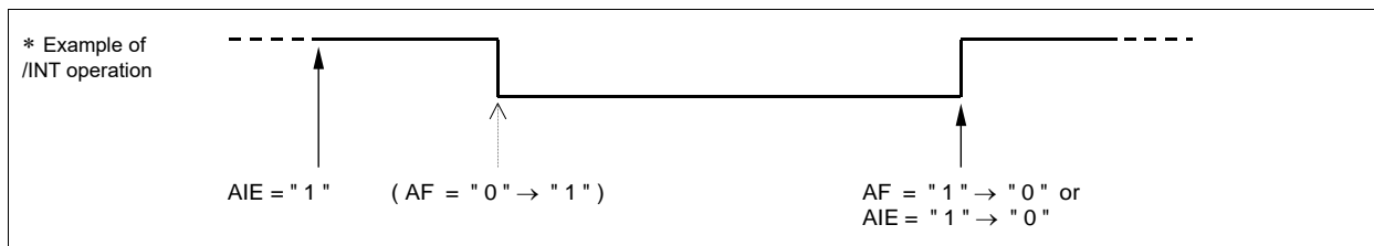
Figure 14 Alarm Function
