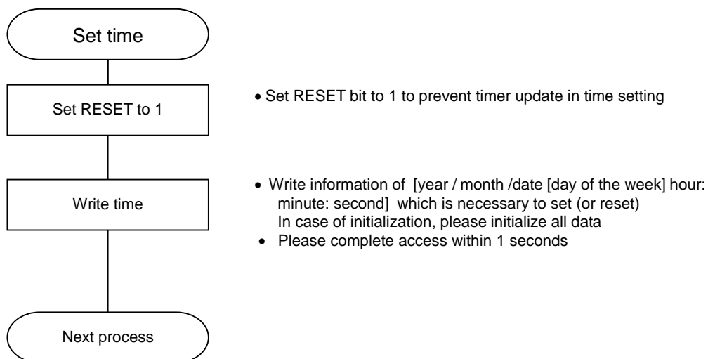
Figure 30 Flow ex. 3
