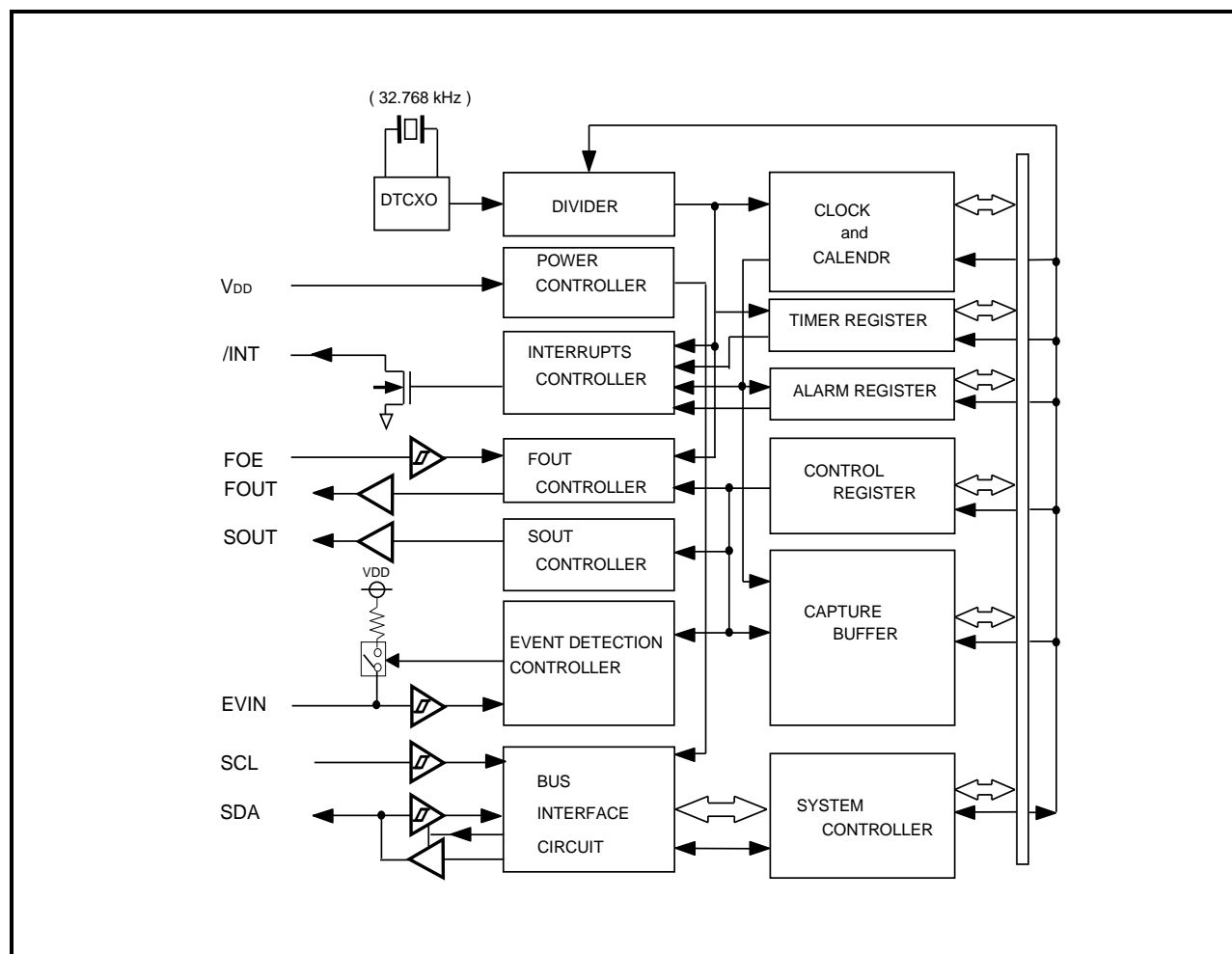
Figure 2 Block Diagram
