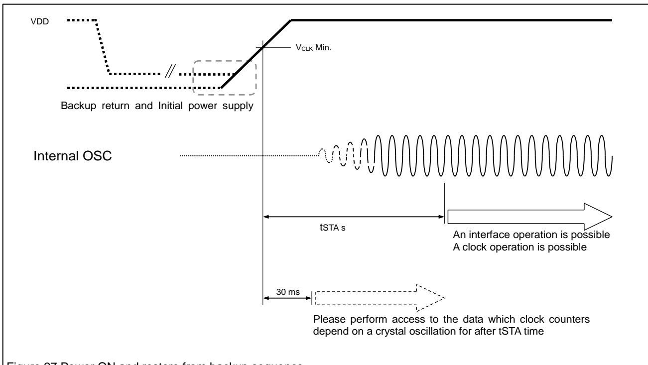
Figure 27 Power ON and restore from backup sequence
