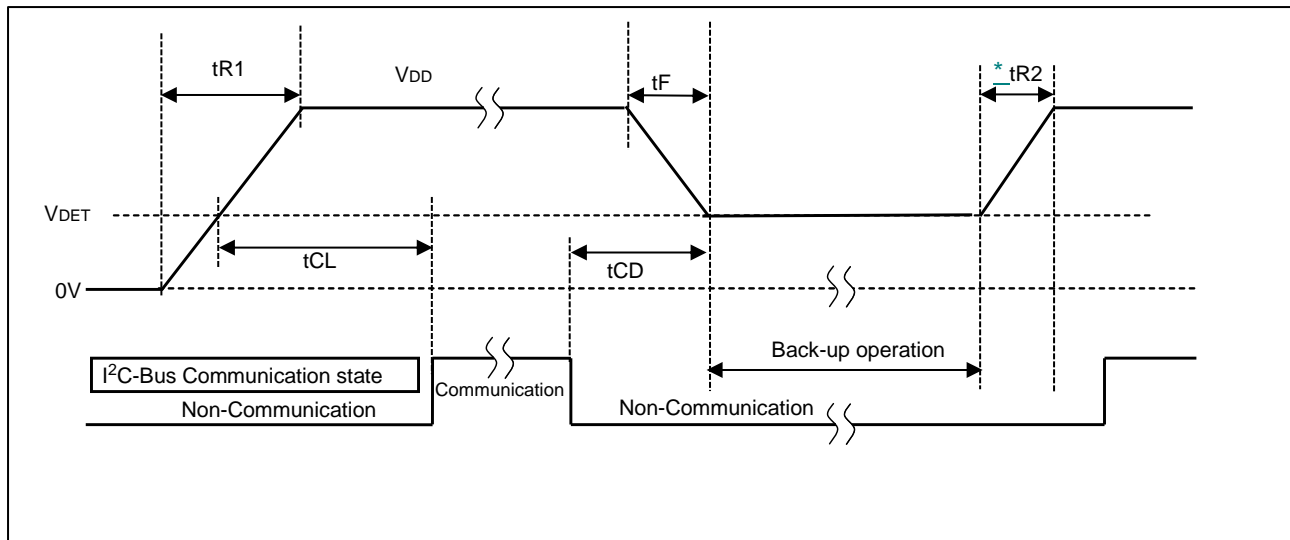
Figure 26 V DD Sequence
