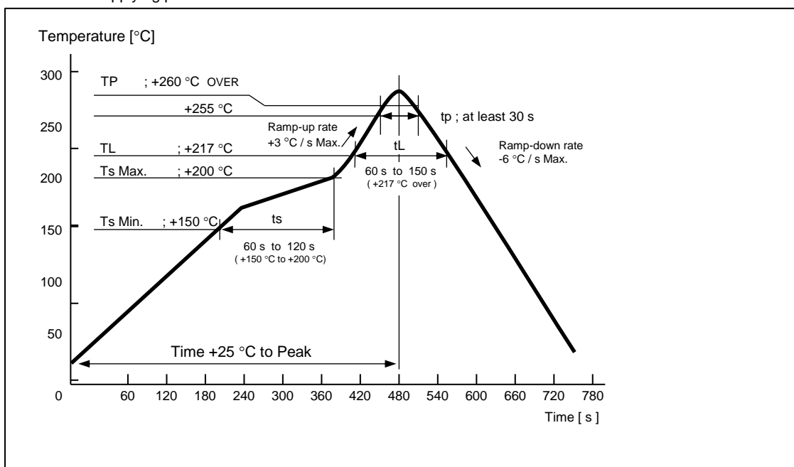
Figure 36 Soldering Profile
