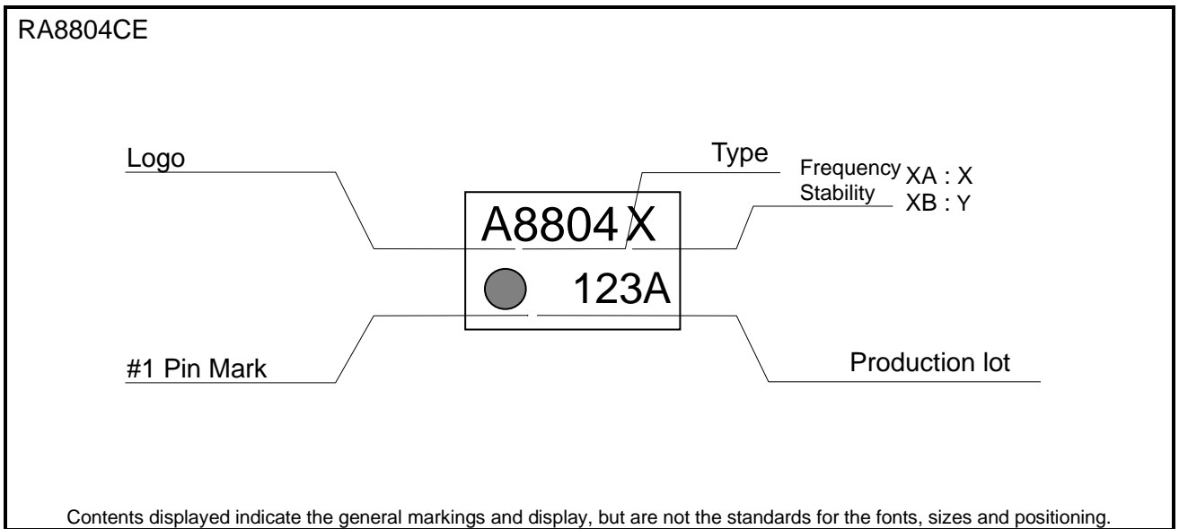
Figure 35 Marking
