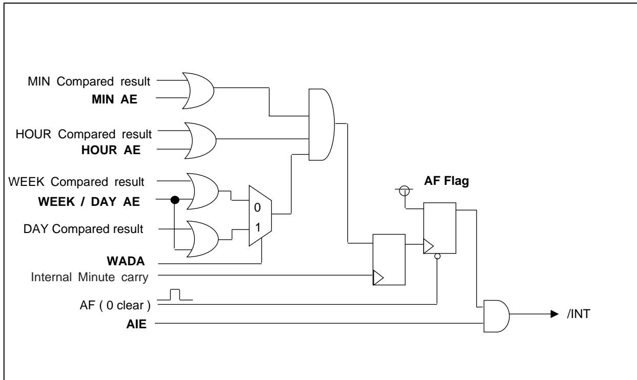
Figure 13 Alarm interrupt block diagram
