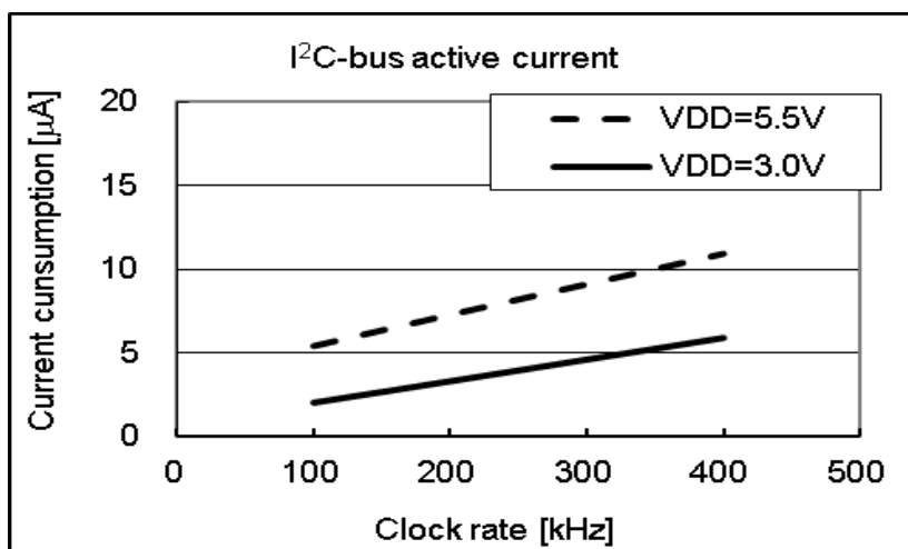
Figure 6 I 2 C-Bus Current consumption
