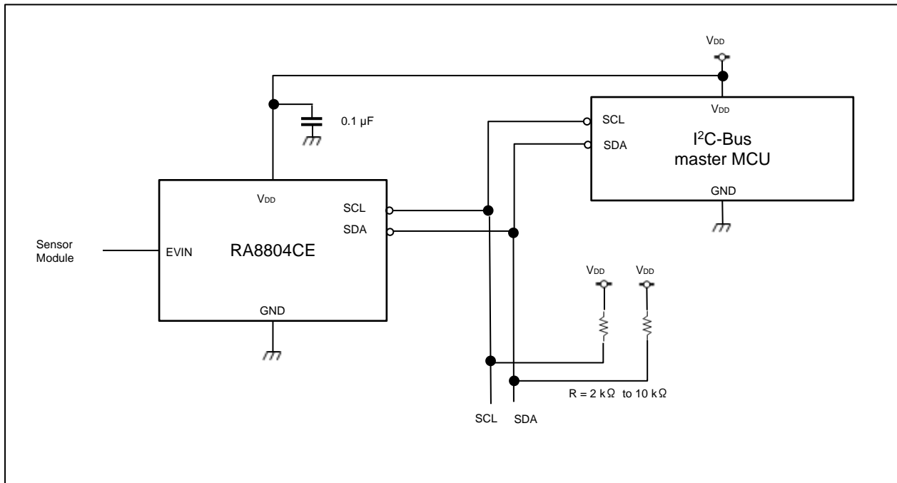
Figure 32 Circuit Diagram
