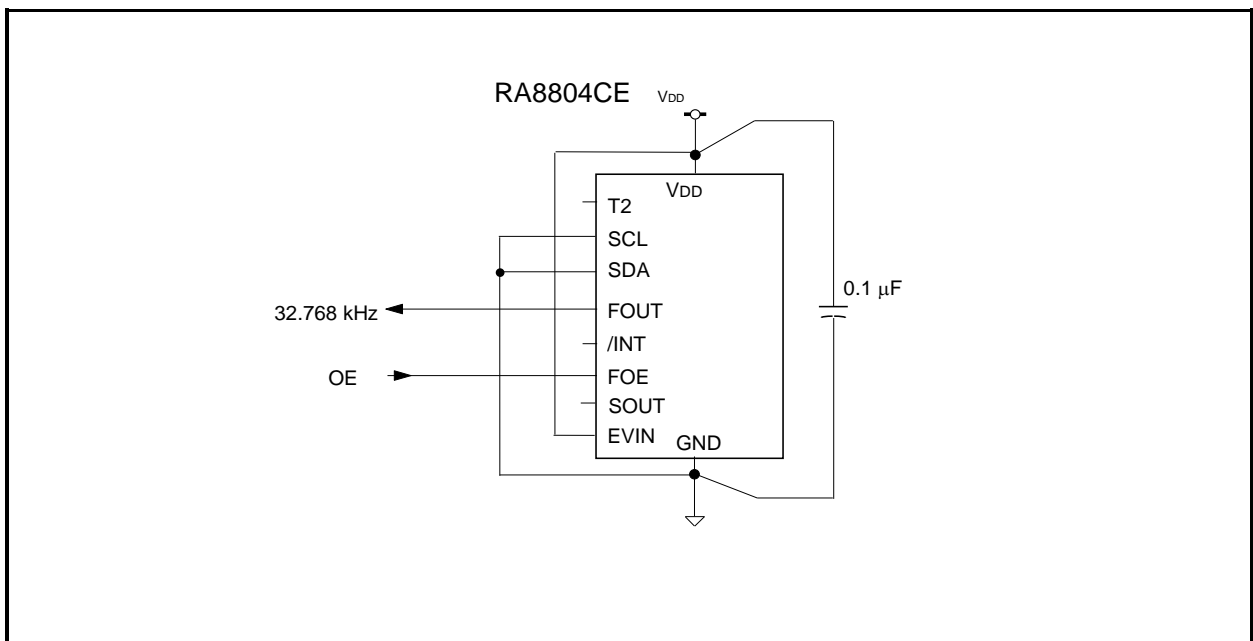
Figure 33 32.768 kHz DTCXO Connection
