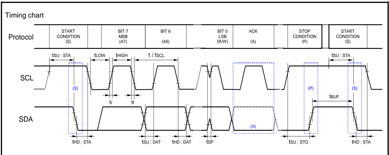
Figure 4 I 2 C-Bus Timing Chart
