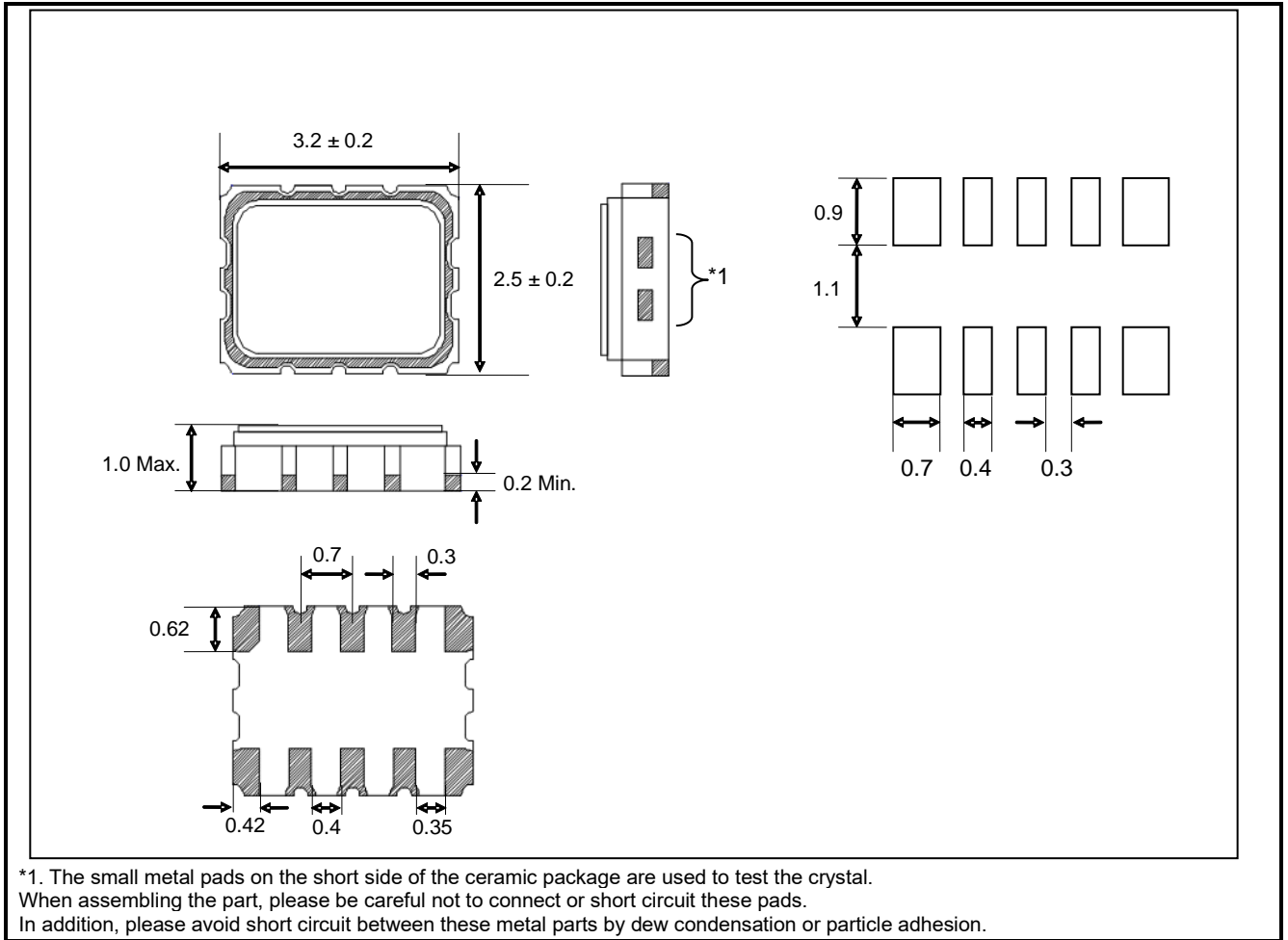
Figure 34 Package Dimension
