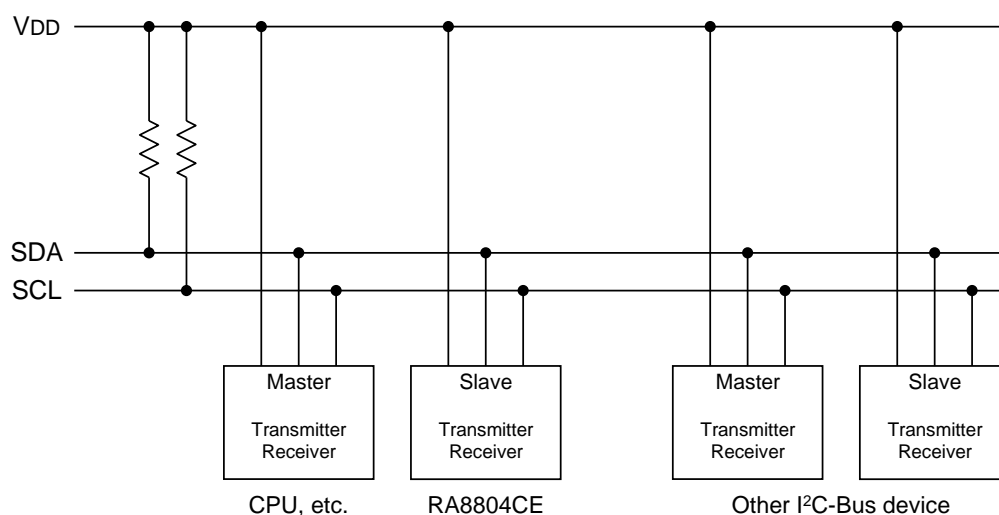
Figure 21 I 2 C-Bus Connection
