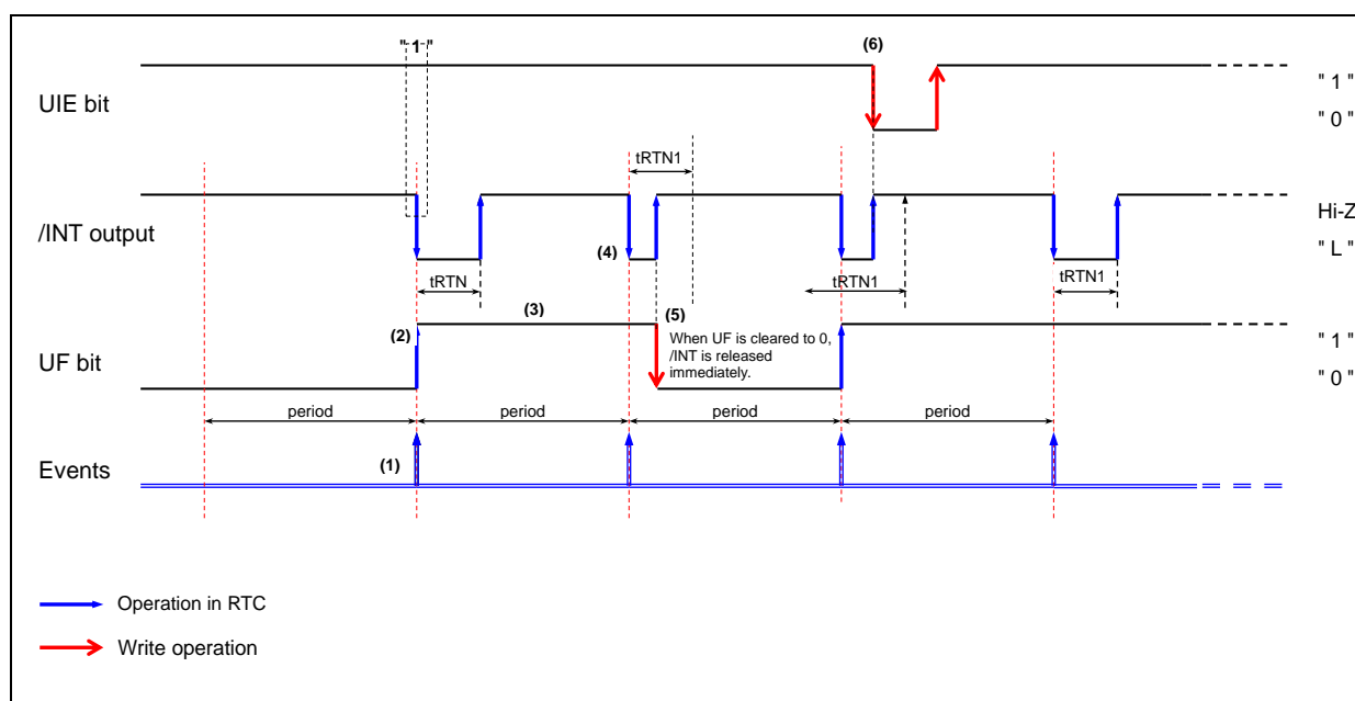
Figure 20 Update Interrupt Timing Chart
