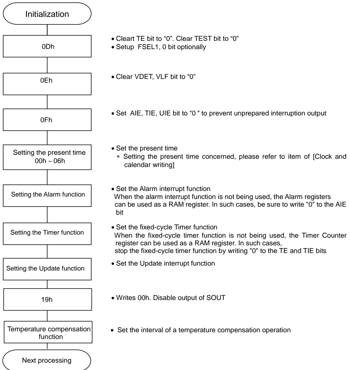
Figure 28 Flow ex. 1
