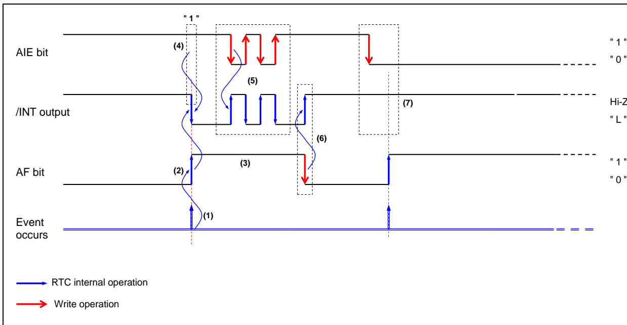
Figure 15 Alarm Timing Chart
