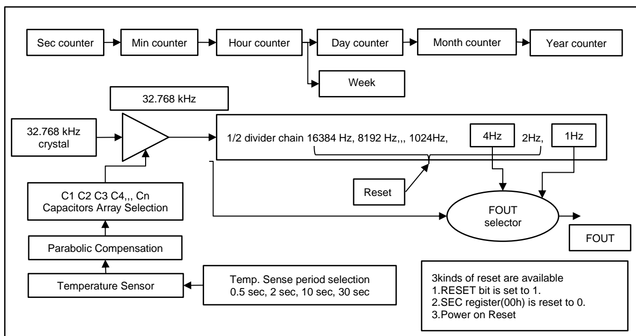
Figure 7 Internal clock distribution diagram
