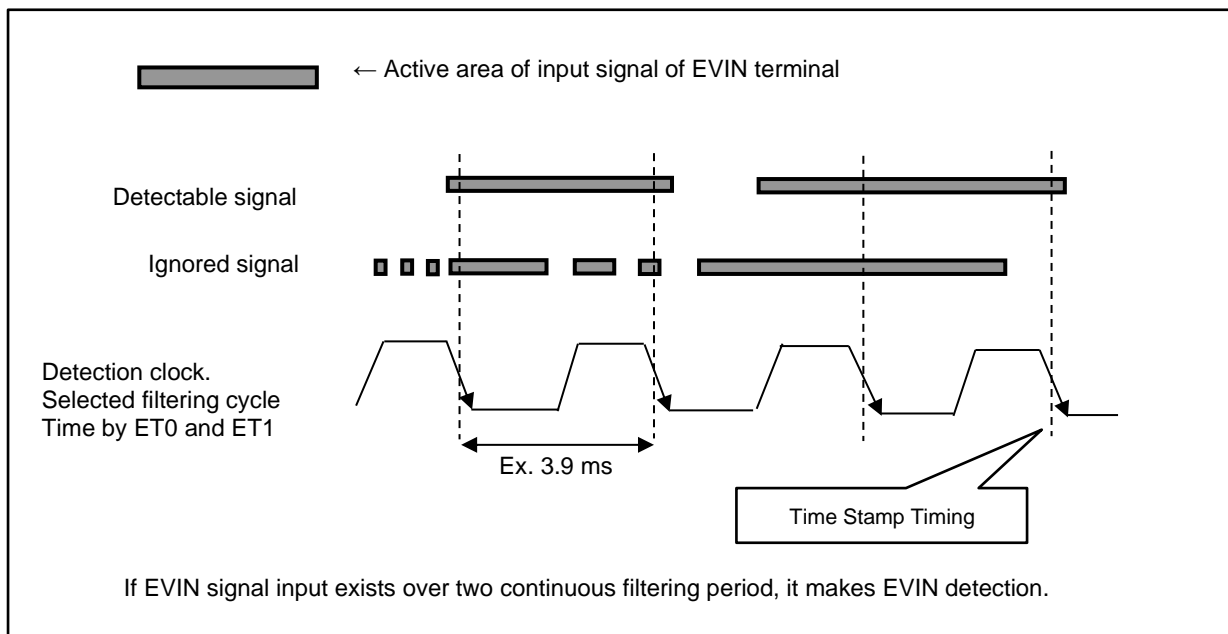
Figure 8 EVIN Debounce Function
