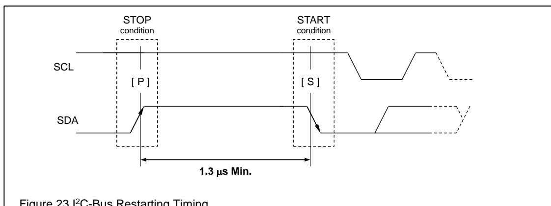
Figure 23 I 2 C-Bus Restarting Timing
