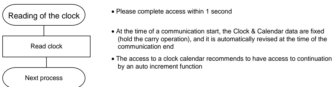
Figure 31 Flow ex. 4
