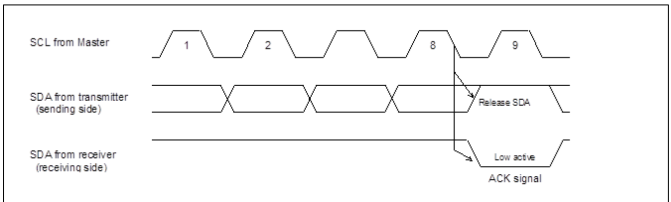
Figure 25 I 2 C-Bus Acknowledge Signal
