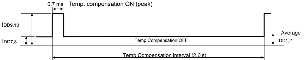
Figure 5 Temperature compensation current
