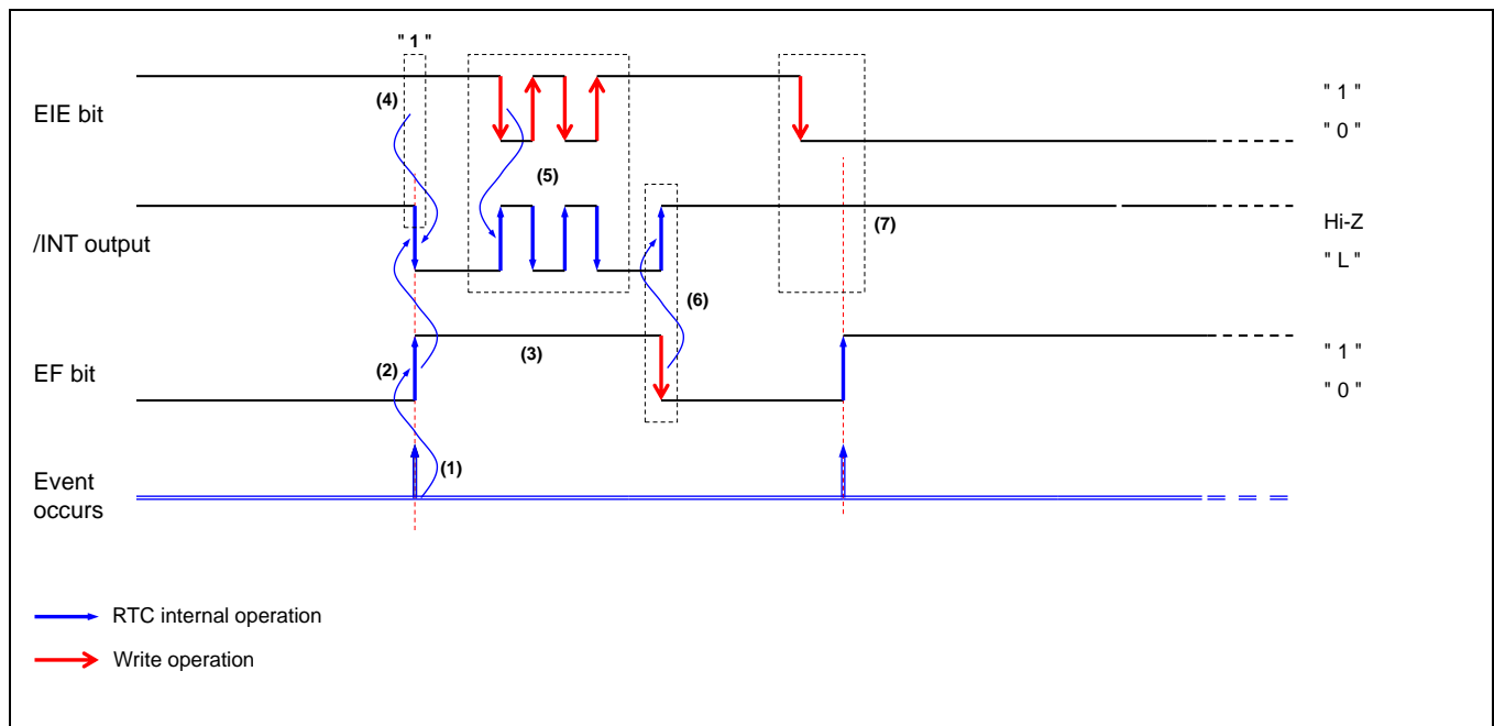
Figure 12 EVIN Timing Chart
