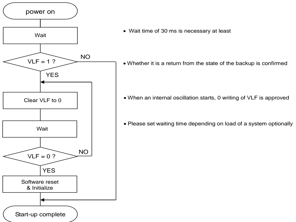
Figure 29 Flow ex. 2
