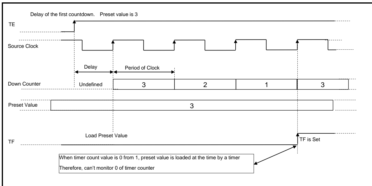
Figure 17 Wakeup Timer Count Down Timing Chart
