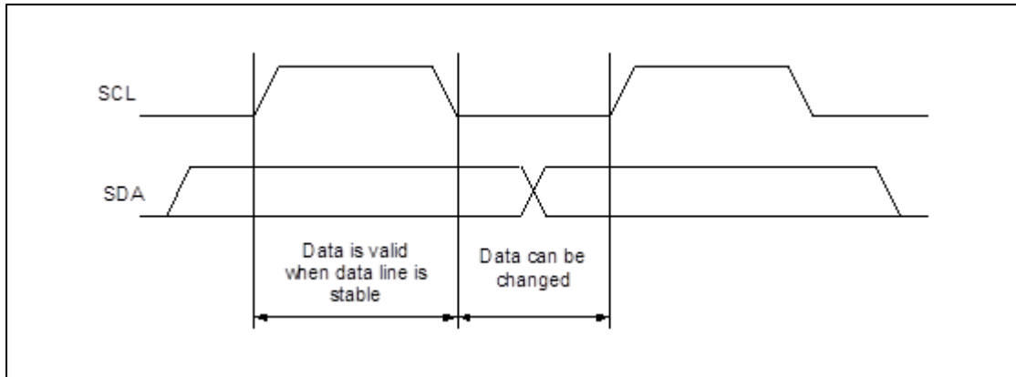
Figure 24 I 2 C-Bus SDA, SCL
