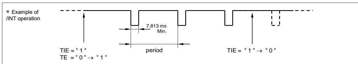
Figure 16 Wakeup Timer Function
