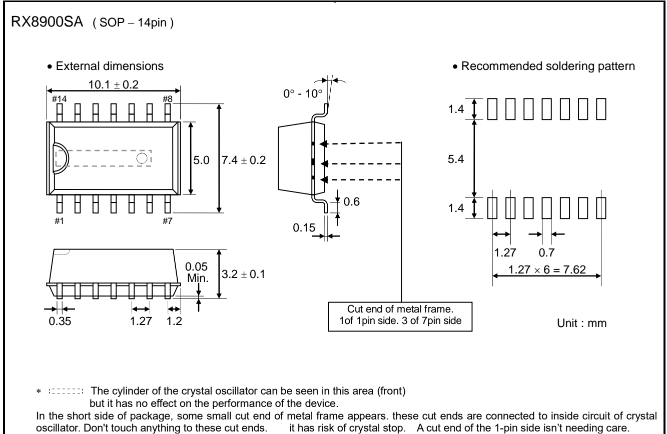
Figure 46 RX8900SA package
