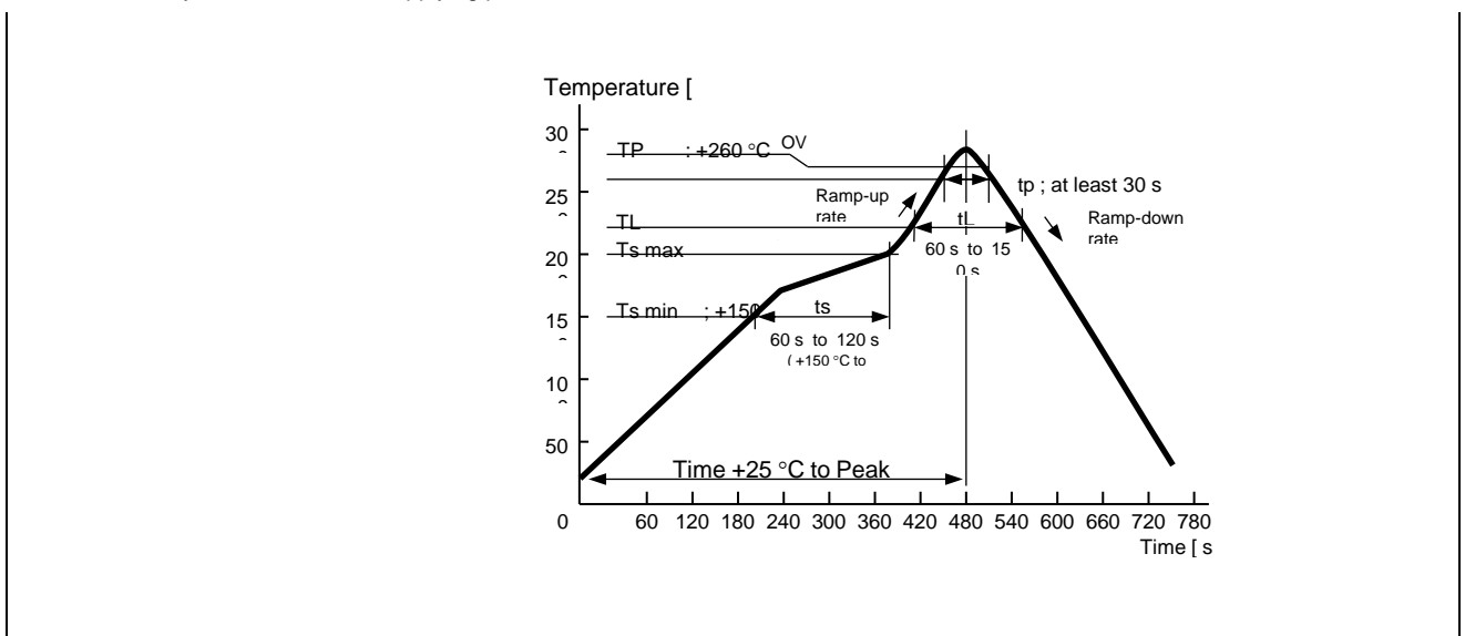
Figure 50 Reference profile
