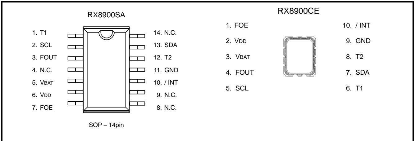
Figure 2 Terminal connections
