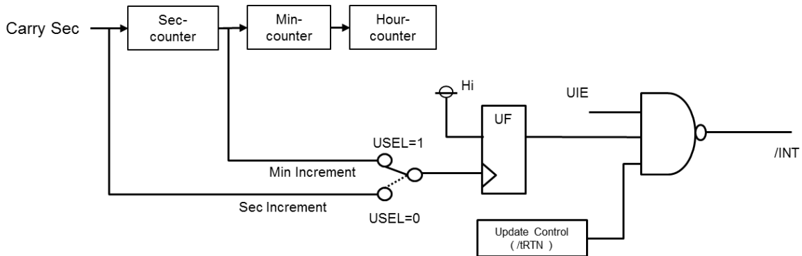
Figure 14 Time Update Interrupt Block Diagram
