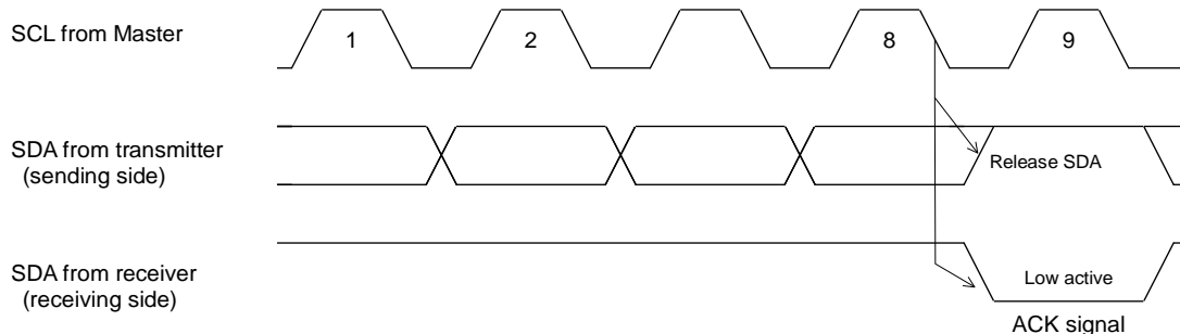
Figure 34 I 2 C bus data acknowledge response
