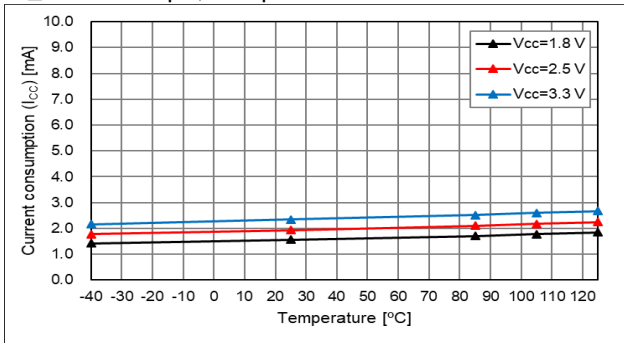
L_{CMOS} = 5\text{ pF} , Temperature Characteristic
