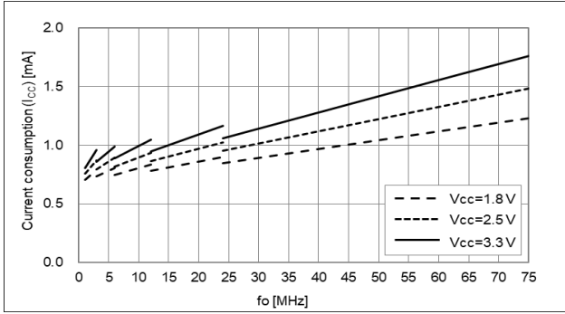
No load, T_{use} = +25\text{ }^{\circ}\text{C} , Freq. Dependency
