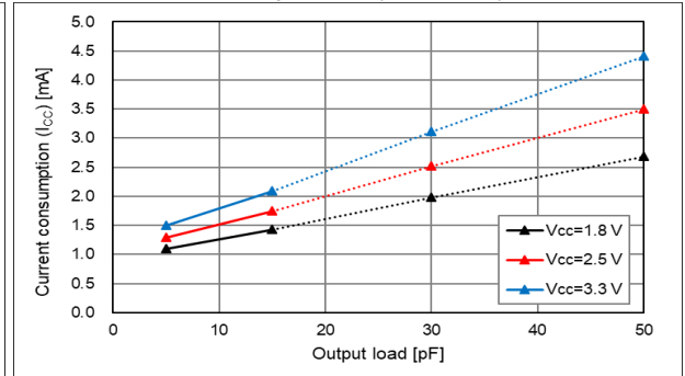
T_{use} = +25\text{ }^{\circ}\text{C} , Output load ( L_{CMOS} ) Characteristics
