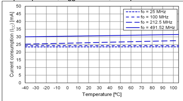
Output option:B, V_{CC} = 2.25 V, Temp. Character
