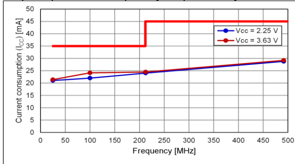
Output option:A, Frequency Dependency
