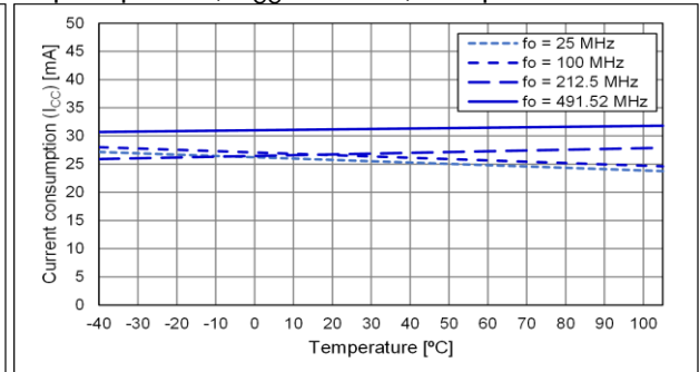
Output option:B, V_{CC} = 3.63 V, Temp. Characteristic
