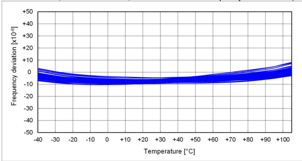
Output option:A, Frequency Dependency
