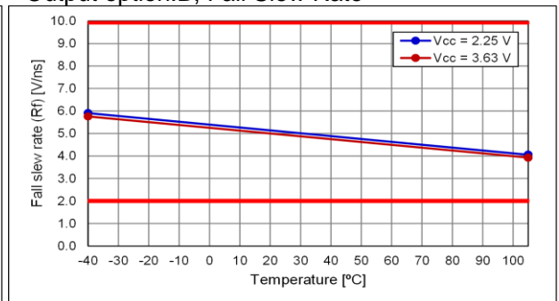
Output option:B, Fall Slew Rate
