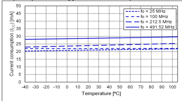
Output option:A, V_{CC} = 2.25 V, Temp. Character
