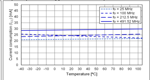
Output option:A, V_{CC} = 3.63 V, Temp. Characteristic
