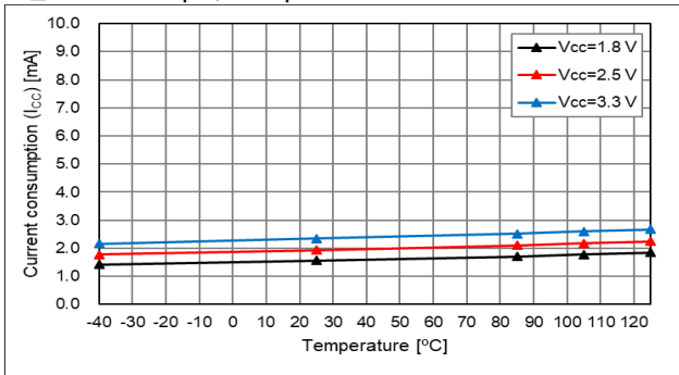
L CMOS = 5 pF, Temperature Characteristic
