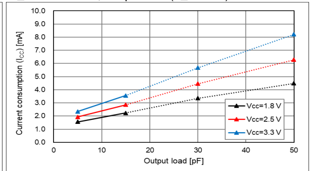
T use = +25 °C, Output load(L CMOS ) Characteristics
