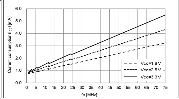
L CMOS = 15 pF, T use = +25 °C, Freq. Dependency
