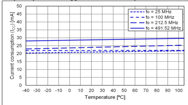
Output option:A, V_{CC} = 2.25 V, Temp. Characteristic
