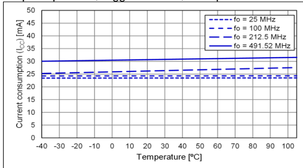
Output option:B, V_{CC} = 2.25 V, Temp. Characteristic
