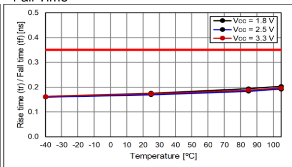
Fall Time
