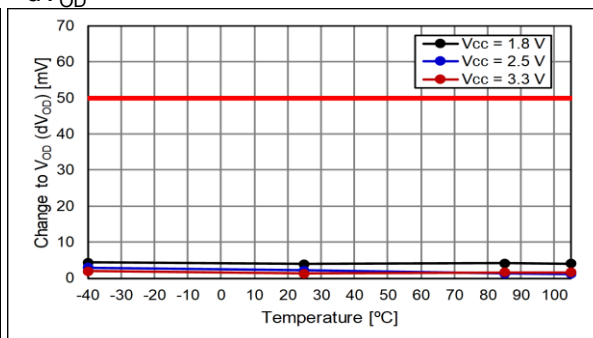
dV_{OD}
