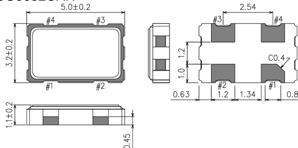
SG5032CAN
