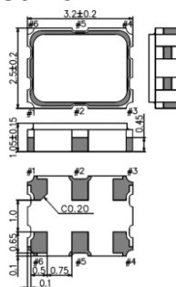
SG3225VEN
