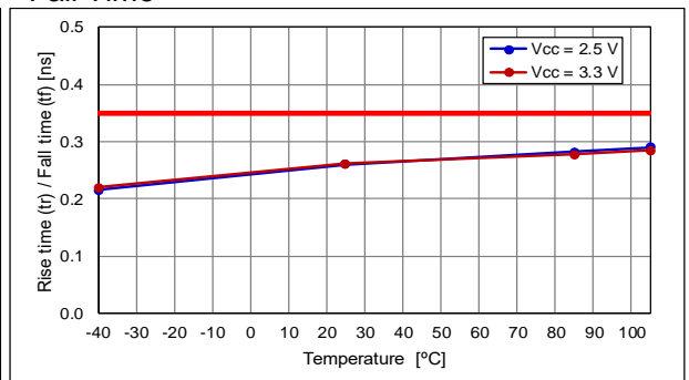
Fall Time
