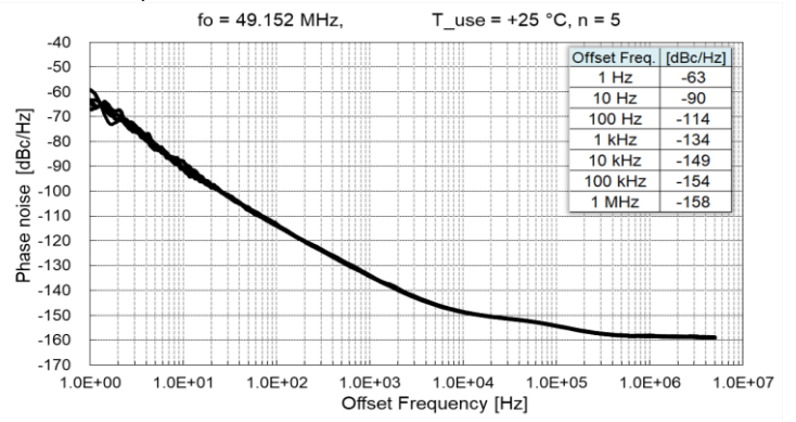
11) fo = 49.152 MHz
