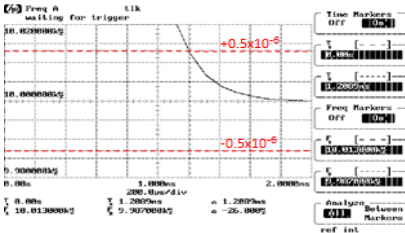
(6-7) Start-up time ( T_{\text{use}} = +25 \text{ }^\circ\text{C} , X axis Scale = 0.2 ms/div)
