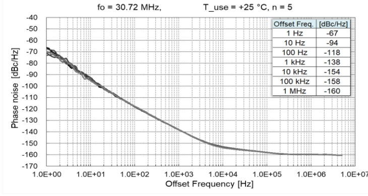
5) fo = 30.72 MHz
