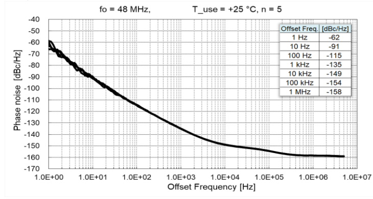
7) fo = 48 MHz
