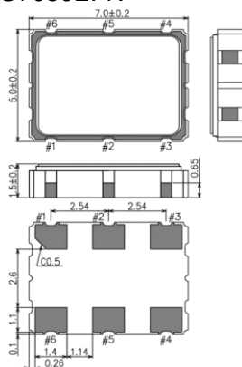
VG7050EFN
