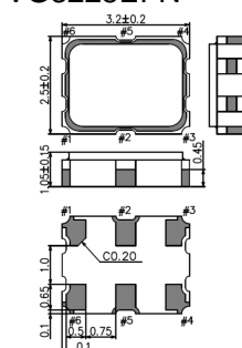
VG3225EFN
