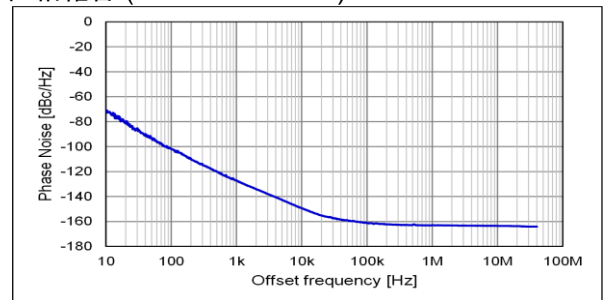
位相雑音 (fo = 122.88 MHz)
