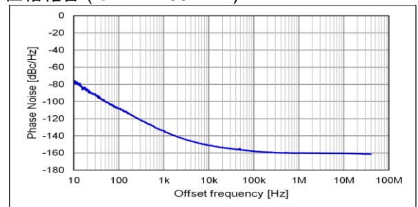
位相雑音 (fo = 122.88 MHz)
