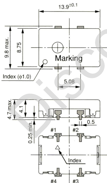
Pin connections
