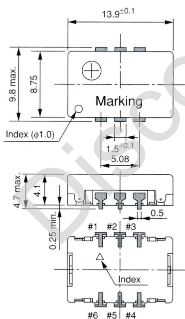
Pin connections
