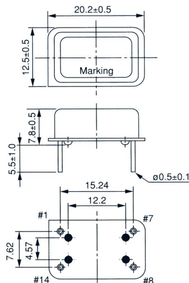
Pin connections
