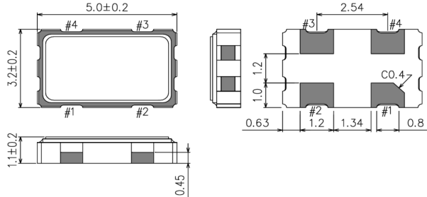
SG5032CAN
