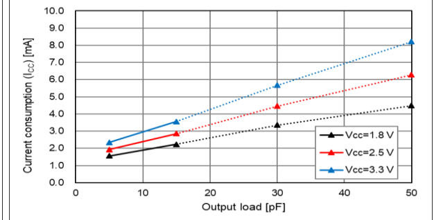
T_{use} = +25\text{ }^{\circ}\text{C} , Output load( L_{CMOS} ) Characteristics
