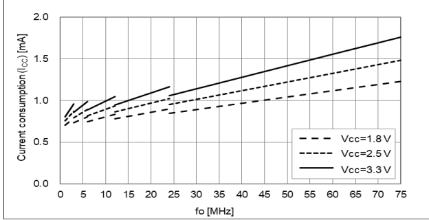
No load, T_{use} = +25\text{ }^{\circ}\text{C} , Freq. Dependency
