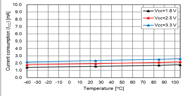
L_{CMOS} = 5\text{ pF} , Temperature Characteristic
