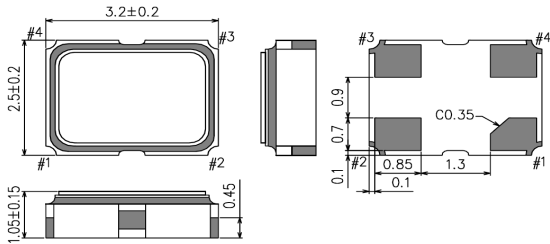
SG3225CAN
