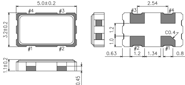
Terminal Assignment
