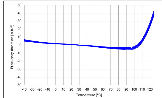
±100 × 10 -6 / -40 °C to +125 °C
