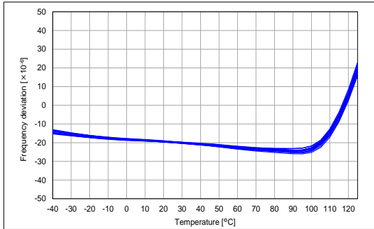
±50 × 10 -6 / -40 °C to +125 °C
