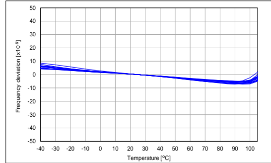
±20 × 10 -6 / -40 °C to +105 °C
