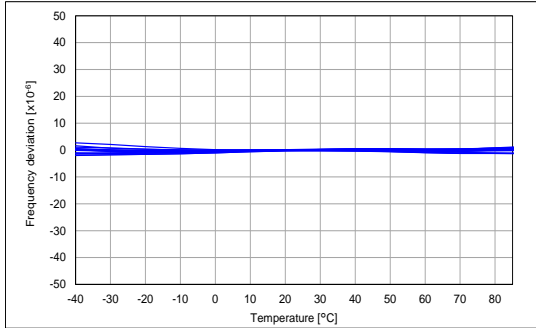
±15 × 10 -6 / -40 °C to +85 °C
