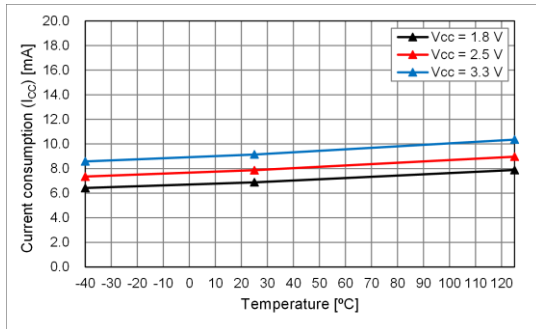
fo = 125 MHz
