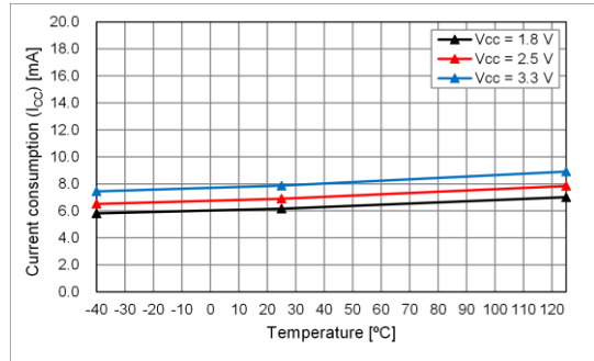
fo = 100 MHz
