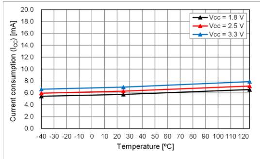
fo = 75 MHz
