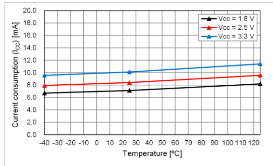
fo = 150 MHz
