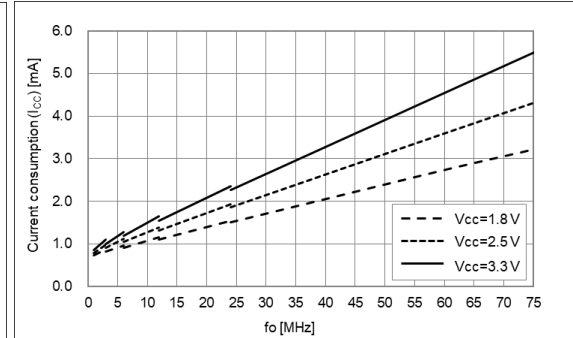
L CMOS = 15 pF, T use = +25 °C, Freq. Dependency
