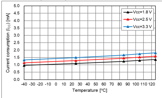
L CMOS = 5 pF, Temperature Characteristic
