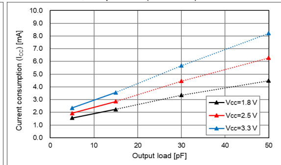
T use = +25 °C, Output load(L CMOS ) Characteristics
