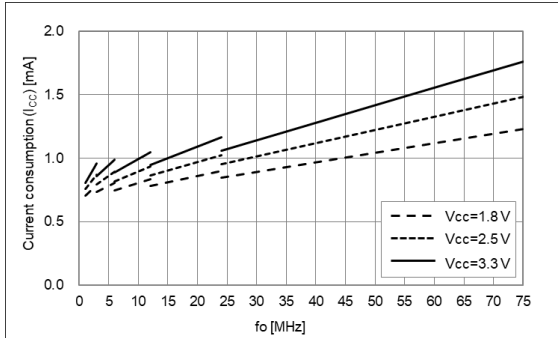
No load, T use = +25 °C, Freq. Dependency
