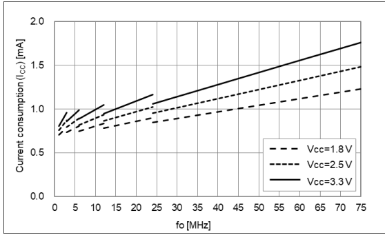
No load, T use = +25 °C, Freq. Dependency
