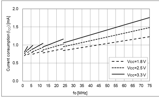
No load, T_{use} = +25\text{ }^{\circ}\text{C} , Freq. Dependency
