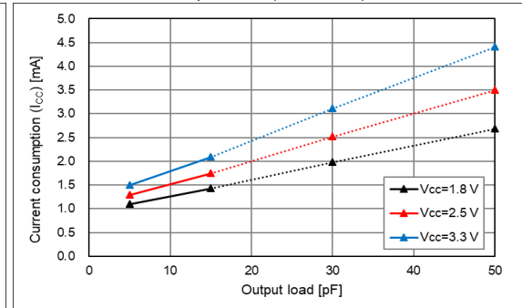
T_{use} = +25\text{ }^{\circ}\text{C} , Output load( L_{CMOS} ) Characteristics
