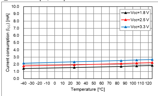
L_{CMOS} = 5\text{ pF} , Temperature Characteristic
