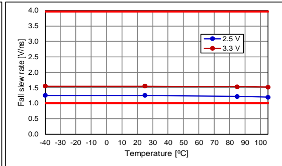
Fall Slew Rate
