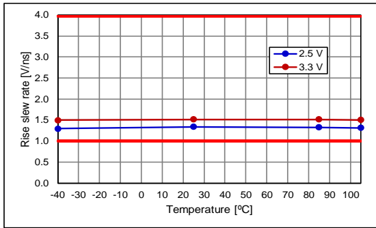
Rise Slew Rate
