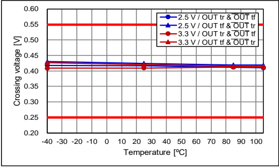
fo = 100 MHz
