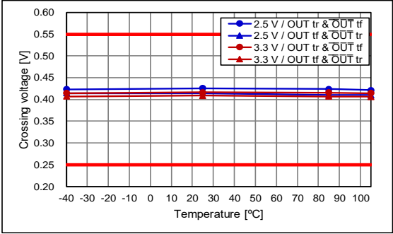
fo = 322.265625 MHz
