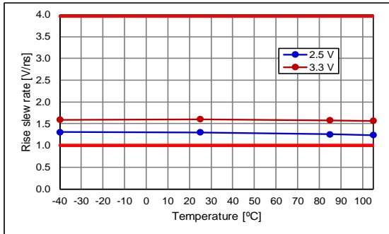
Rise Slew Rate
