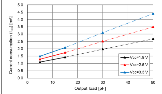
T_{use} = +25\text{ }^{\circ}\text{C} , Output load( L_{CMOS} ) Characteristics
