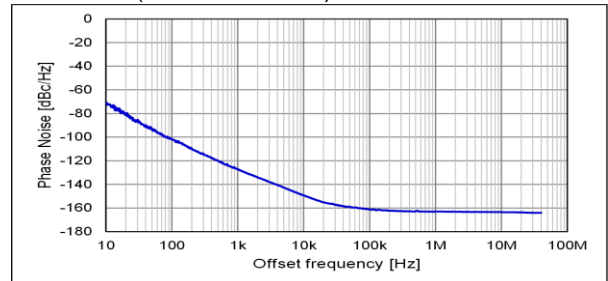
Phase Noise (fo = 122.88 MHz)
