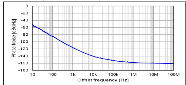
Phase Noise (fo = 491.52 MHz)
